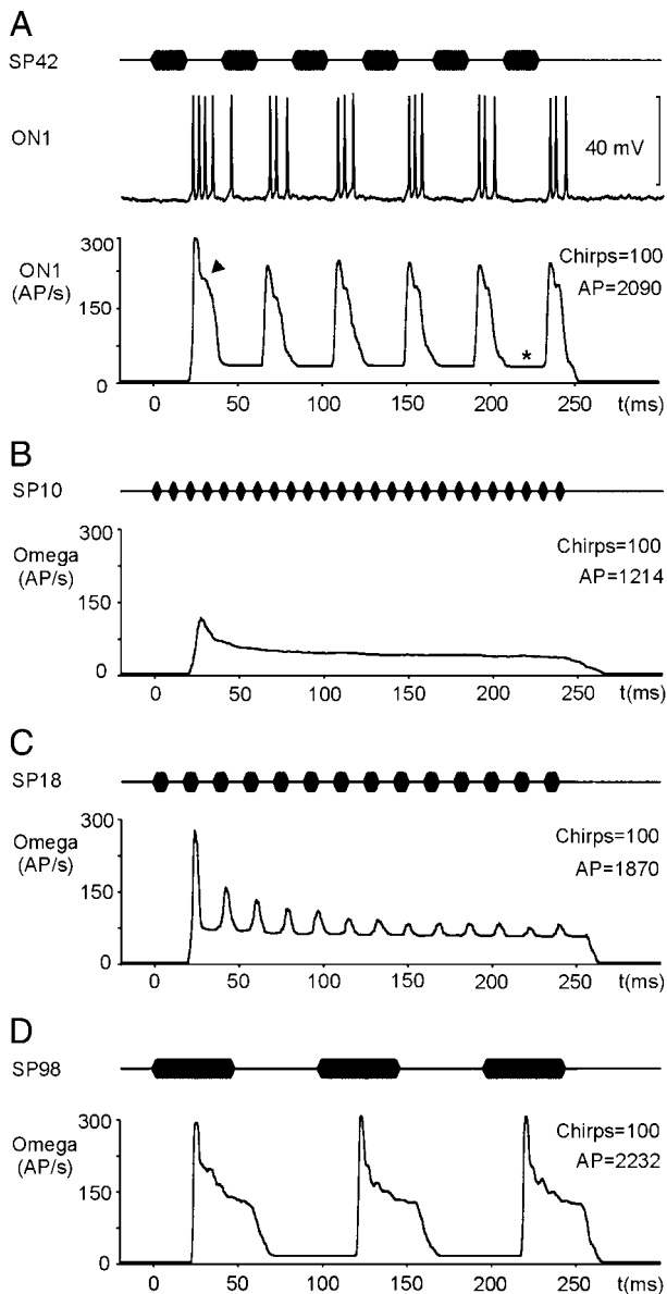
FIG. 2. A : axonal intracellular recording of Omega neuron (ON1, middle ) when stimulated with the species-specific SP of 42 ms ( top ). Instantaneous spike rate of ON1 ( bottom ) averaged over 100 chirps. B–D : response of an ON1 to sound patterns with different SP. B : a tonic response that does not reflect the syllable pattern is indicated by the averaged instantaneous spike rate when ON1 is stimulated with SP10. C : presentation of SP18 yields spike rate peaks of diminishing amplitude. D : stimulation with SP98 demonstrates at the beginning of each response a sharp maximum in the instantaneous spike rate. All averages are based on 100 chirps.
