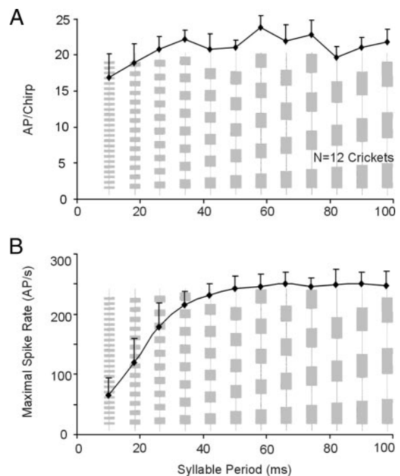
FIG. 3. A : number of action potentials (AP) elicited per chirp plotted against the SP. The erratic change in the curve corresponds to differences in the overall duration of the sound pattern presented at different SPs. B : average maximal peak spike rate of ON1 as elicited by the syllables of each of the different sound patterns. Normalized and pooled data from 12 crickets.
