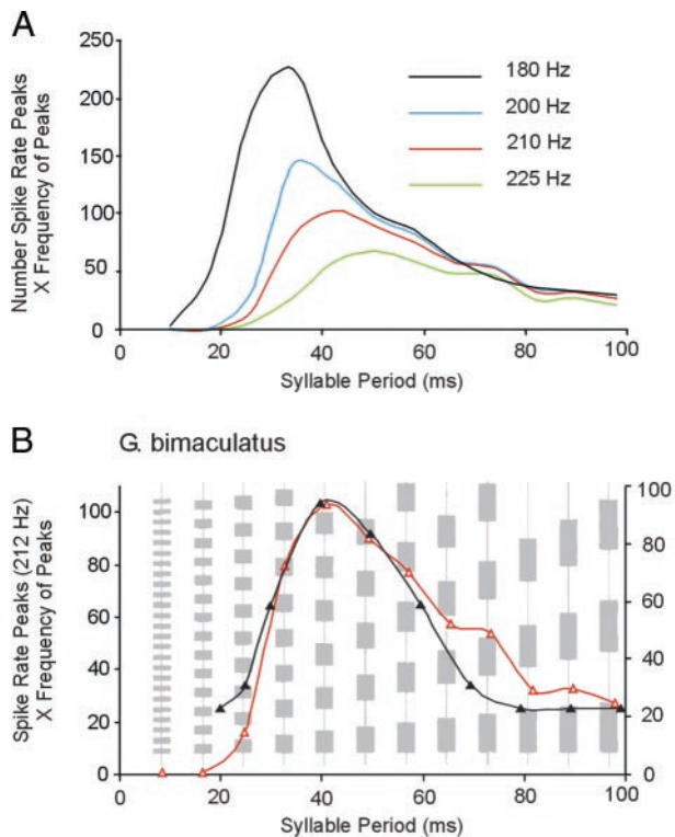
FIG. 5. Comparison of calculated tuning curves with the tuning of phonotactic behavior. A : calculated neural tuning curves for thresholds of 180 Hz (black), 200 Hz (blue), 210 Hz (red), and 225 Hz (green). With increasing threshold, the peak of the tuning curve drops and shifts to longer syllable periods. B : tuning of phonotaxis in crickets walking at 22°C (black line, closed symbols) and calculated neural tuning for discharge peaks of 212 Hz (red line, open symbols). Data for G. bimaculatus phonotaxis are redrawn from Doherty (1985a, Fig. 9).
