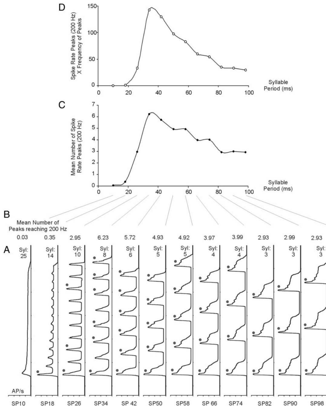
FIG. 4. Calculation of the neuronal tuning corresponding to phonotactic behavior as based on instantaneous spike rate coding. From bottom to top : A , the instantaneous spike rate response of an ON1 to all different SP tested. Time is indicated on the vertical axis. For all stimulus patterns, the number of syllables per chirp is indicated at the upper end of the averages. All spike rate peaks reaching 200 Hz are indicated by a dot. B : table with the mean number of spike rate peaks reaching 200 Hz for all crickets tested. C : number of spike rate peaks reaching 200 Hz plotted against the SPs. The number of spike rate peaks increased to a maximum at SP34 and then decreased in a step like manner to 3 at SP98 closely following the number of syllables per chirp. D : the number of spike rate peaks as given in C is multiplied by the frequency of the spike rate peaks and a band-pass tuning curve similar to the tuning of phonotactic behavior is obtained.
