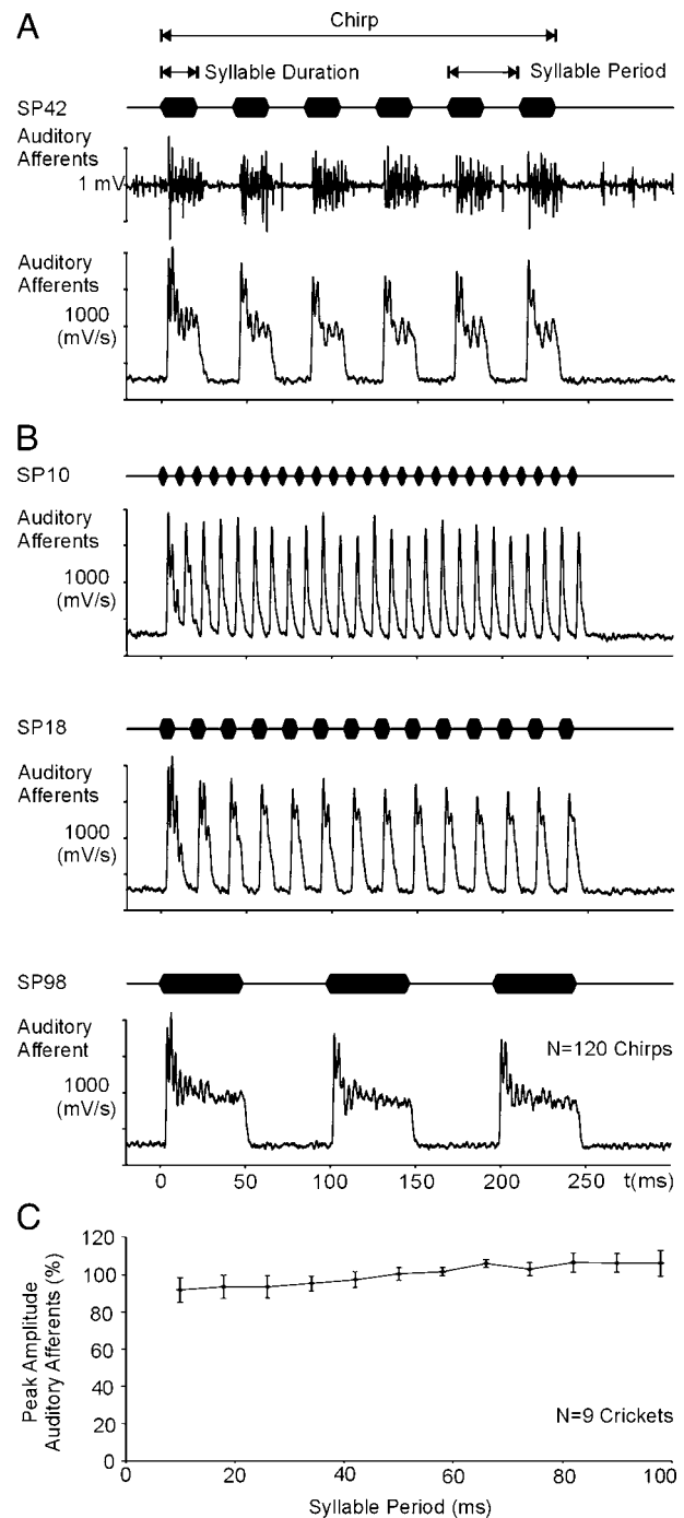
FIG. 1. Summed response of the auditory afferents to sound stimuli of different syllable periods (SP). A : response of the afferents ( middle ) when stimulated with the species-specific SP of 42 ms ( top ) and averaged response after the absolute voltage change of the summed nerve recording ( \sum|dV/dt| ) was calculated ( bottom ). B : sound stimuli ( top ) and averaged afferent response ( bottom ) to SP10, SP18, and SP98. C : peak response of the auditory afferents to stimulation with different syllable periods. Data pooled from 9 crickets and peak responses normalized to the mean (100%). All averages based on 120 chirps.
