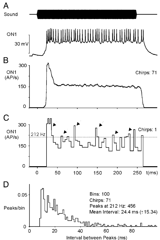
FIG. 6. Responses of ON1 to tone bursts of chirp duration. A : sound pulse (top) and dendritic ON1 recording (bottom). B : the instantaneous spike rate of ON1 averaged over 71 chirps indicates a constant response of the neuron after the initial peak response. C : instantaneous spike rate of ON1 in response to a single tone burst of 250 ms. \cdots , a spike rate of 212 Hz; \downarrow , spike rate peaks that reach 212 Hz. D : frequency distribution of the intervals between spike rate peaks reaching 212 Hz. The mean interval is 24.4 ms corresponding to an SP48.8, which is close to the optimum of phonotactic tuning (see Fig. 5B).
